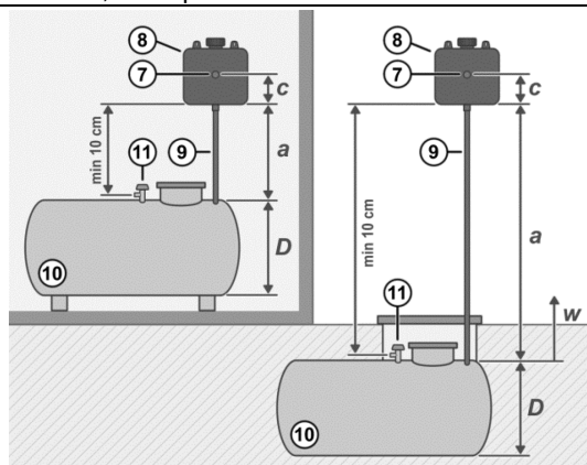
Figure 4: Installation dimensions for the LDL tank, for explanations see Table 6
